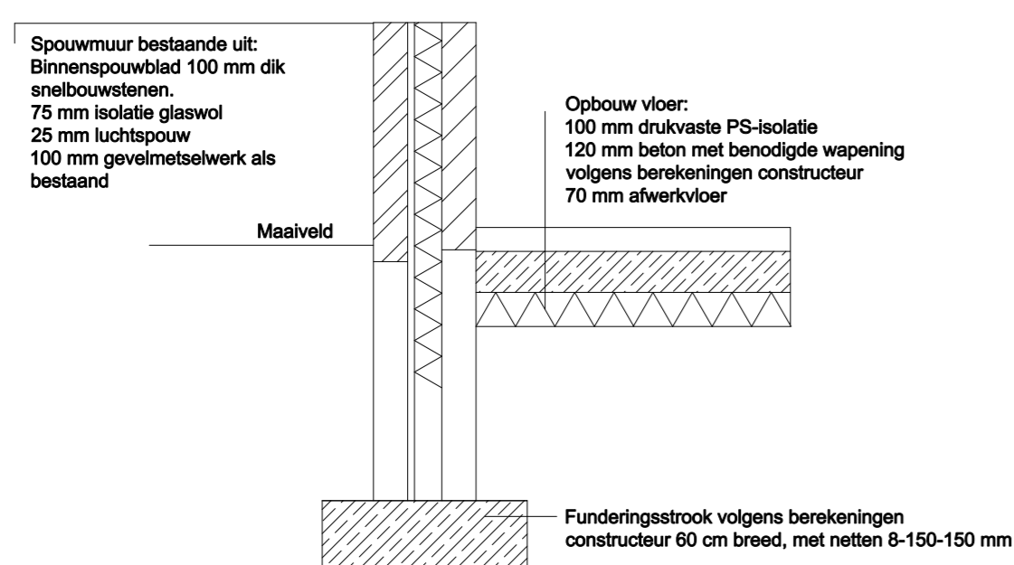
Detail 1
