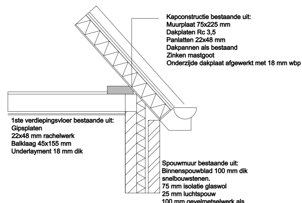
Detail 2
