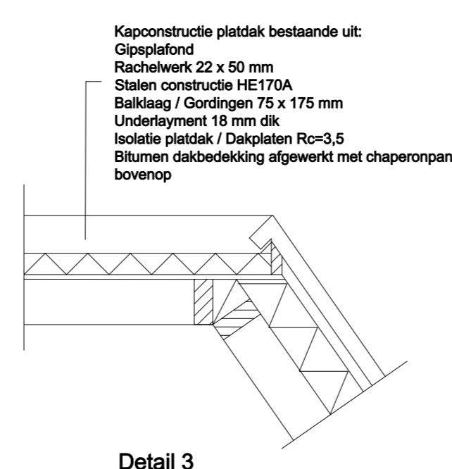
Detail 3
