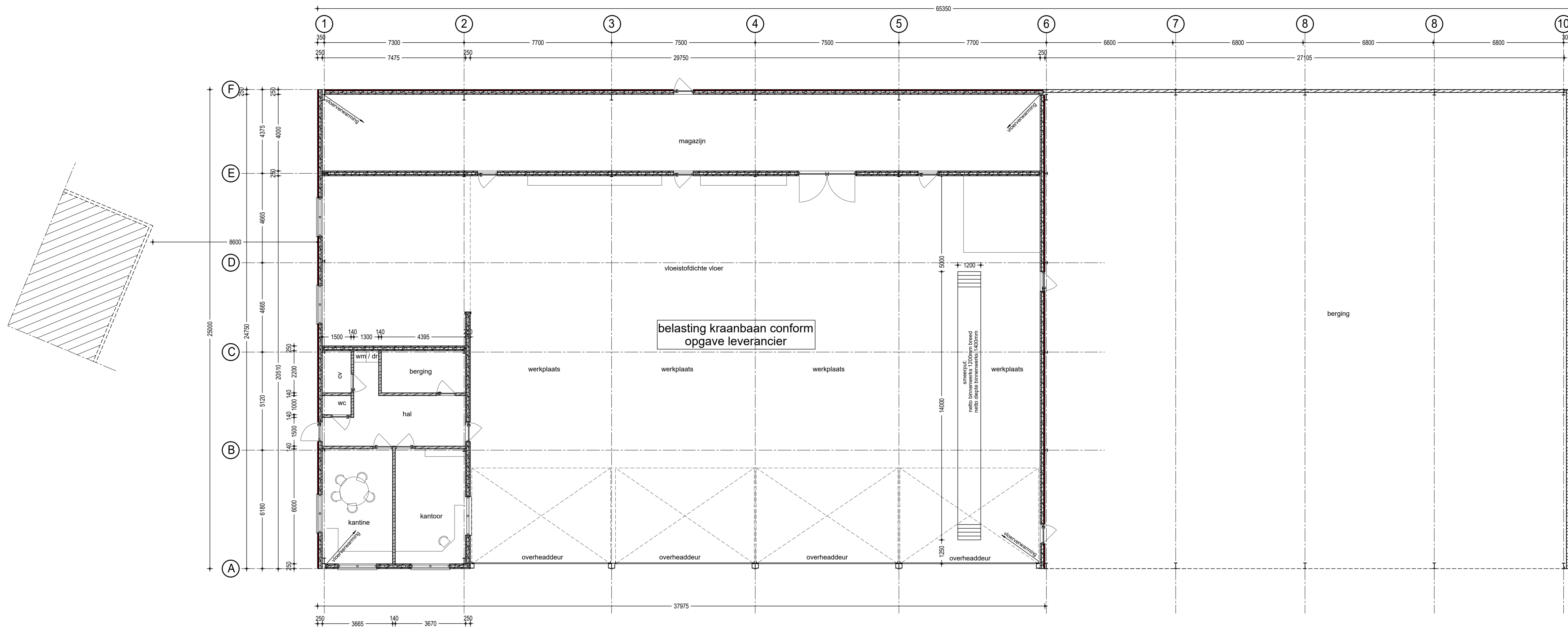
Beganegrond loads 1
