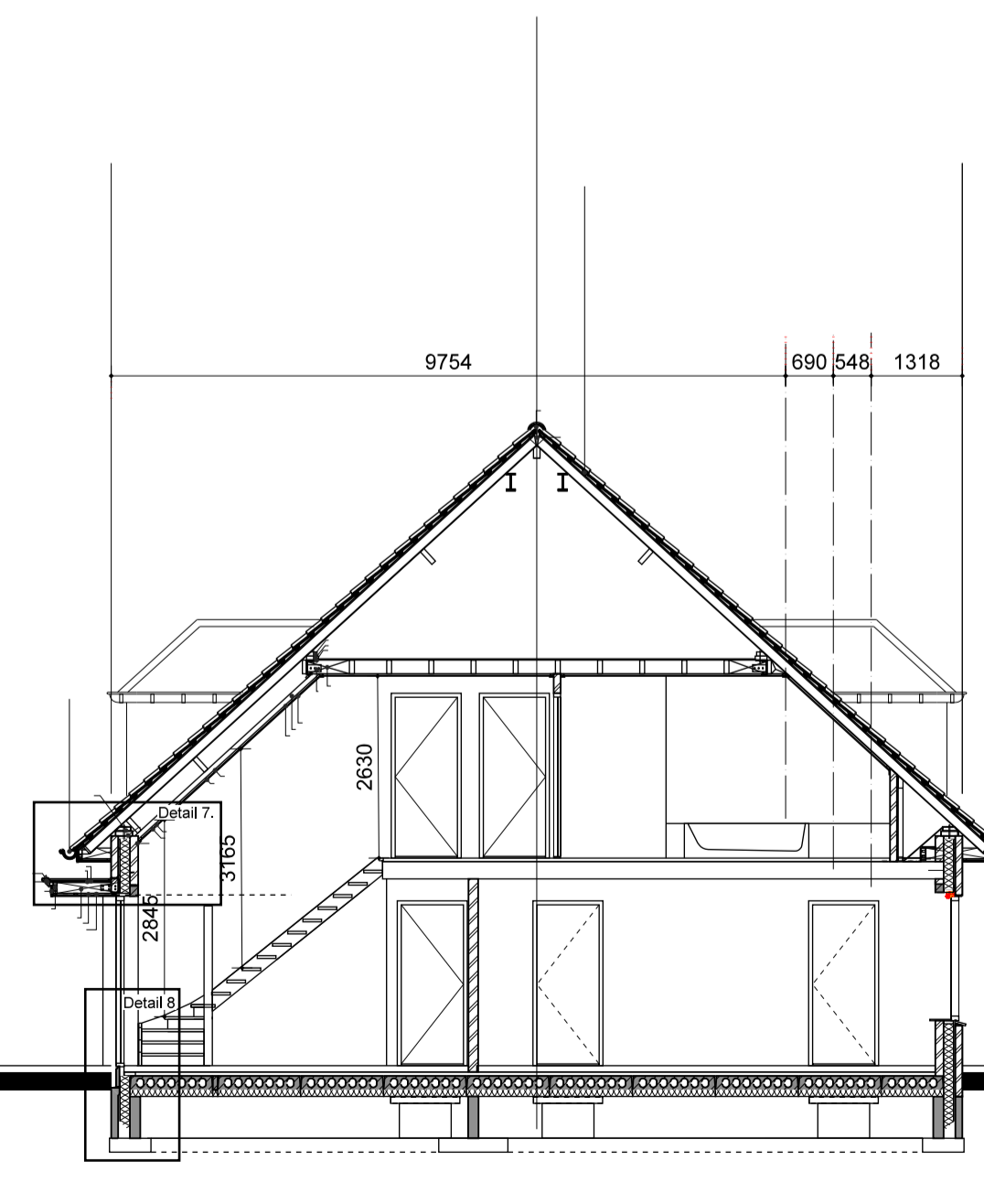
* DOORSNED E B - B *
