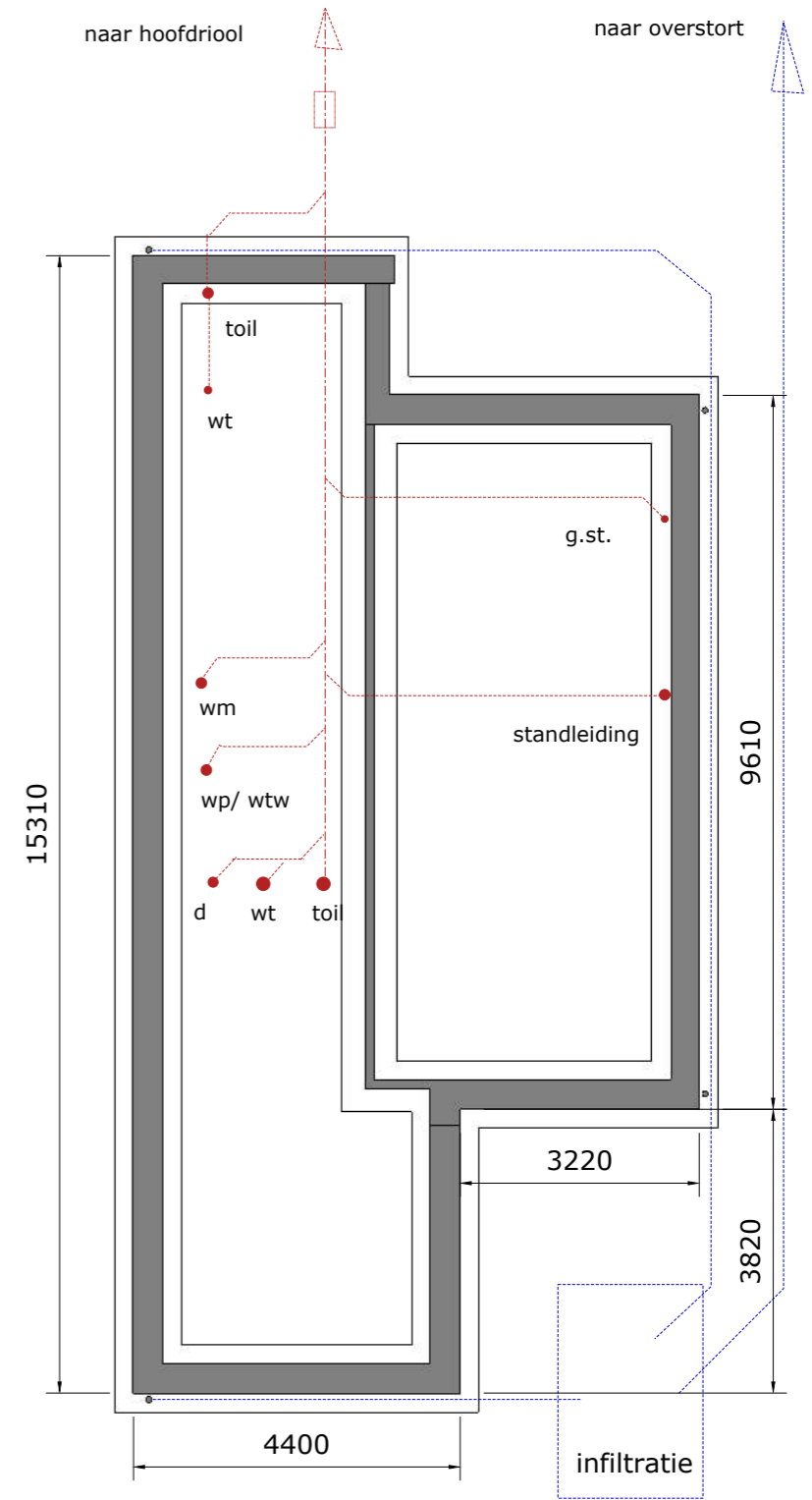
PRINCIPE FUNDERING/RIOLERING
